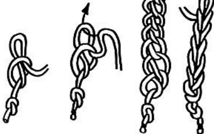
Kettingplakking (chain sinnet)
